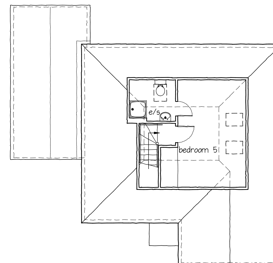
ROOFSPACE PLAN
