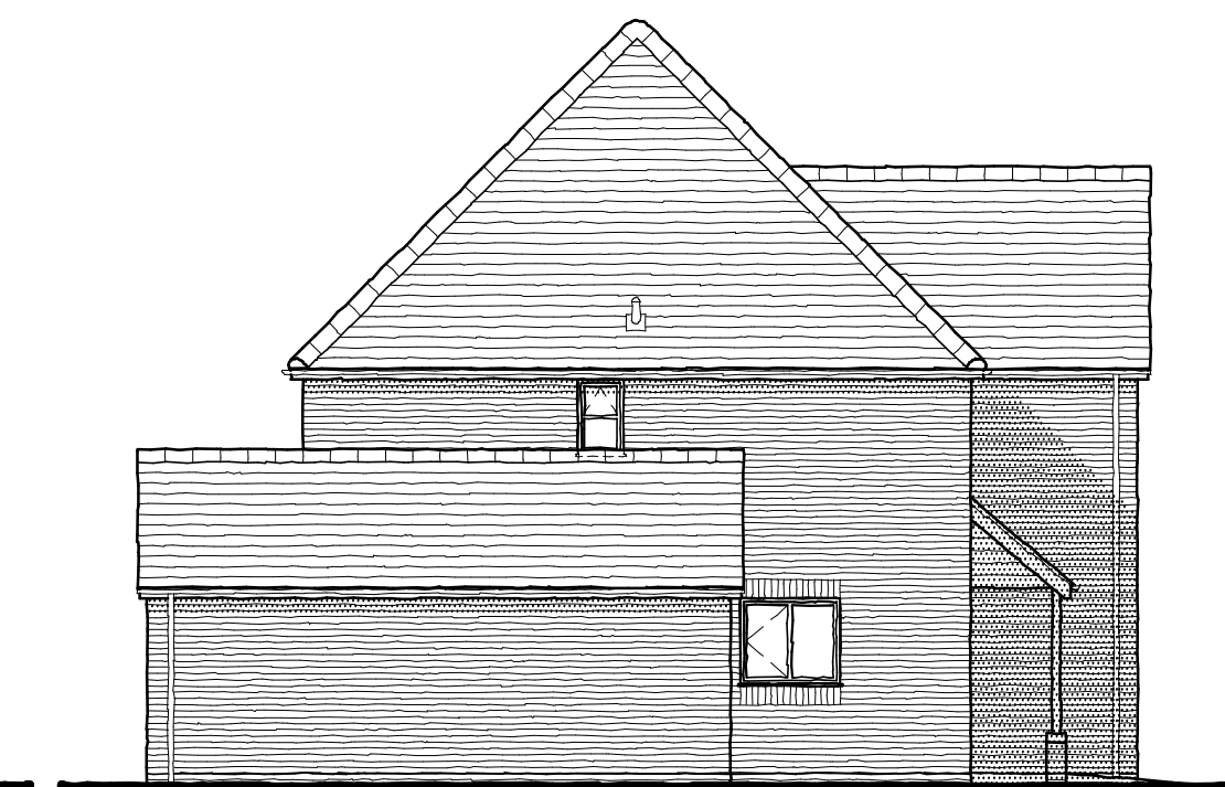
SIDE ELEVATION
