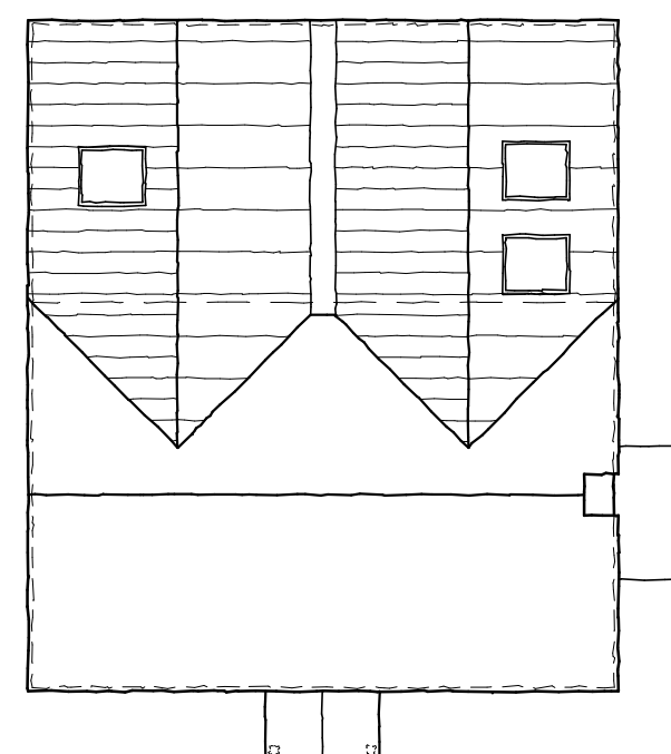
ROOF PLAN
